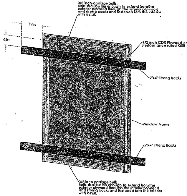
FIGURE A103.1(1) BOARDING OF DOOR OR WINDOW
